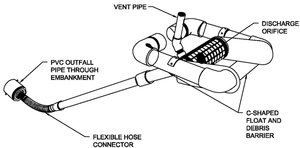
EXAMPLE OF SURFACE SKIMMER N.T.S.
