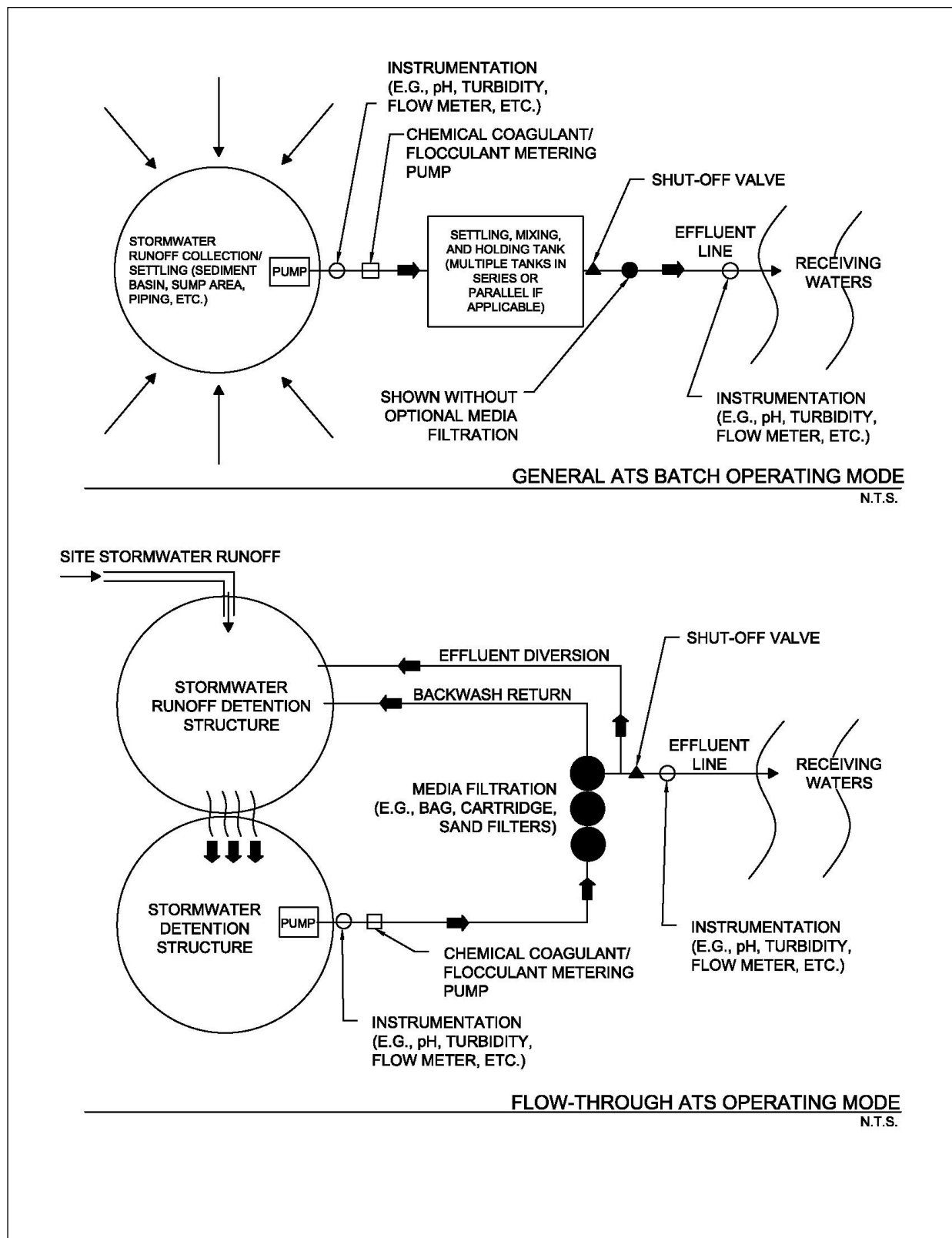
Figure 3.1 Schematics of Active Treatment System
