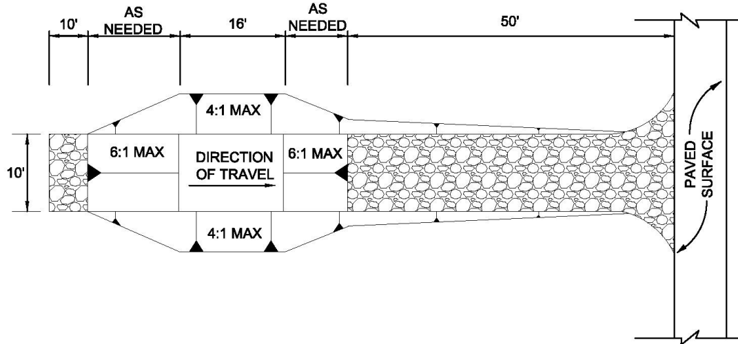
FLOODED BASIN WHEEL WASH PLAN VIEW
